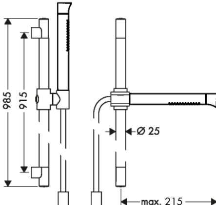
AXOR Starck Organic 12231XX0
