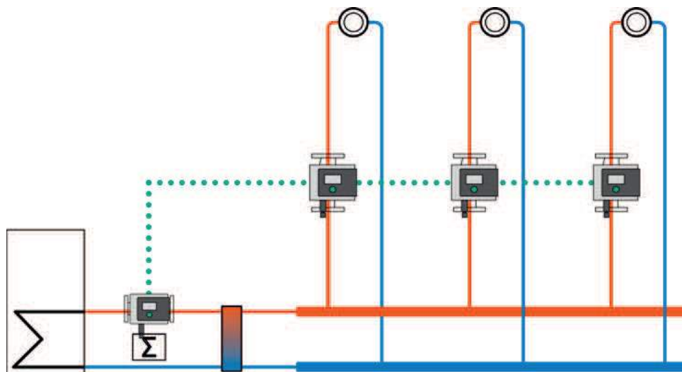
Fig. 29: Multi-Flow Adaptation
