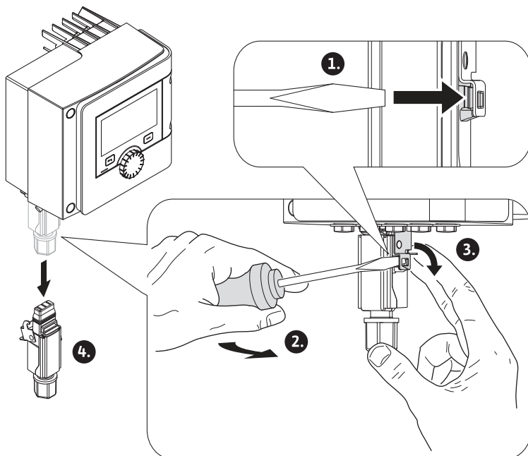
Fig. 12: Wilo-Connector demontieren
