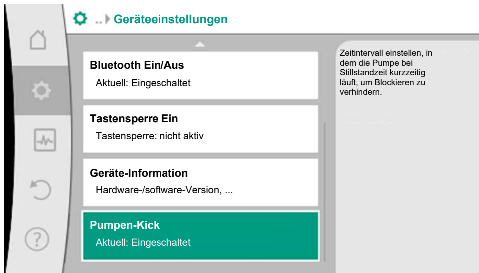
Fig. 88: Pumpen-Kick
