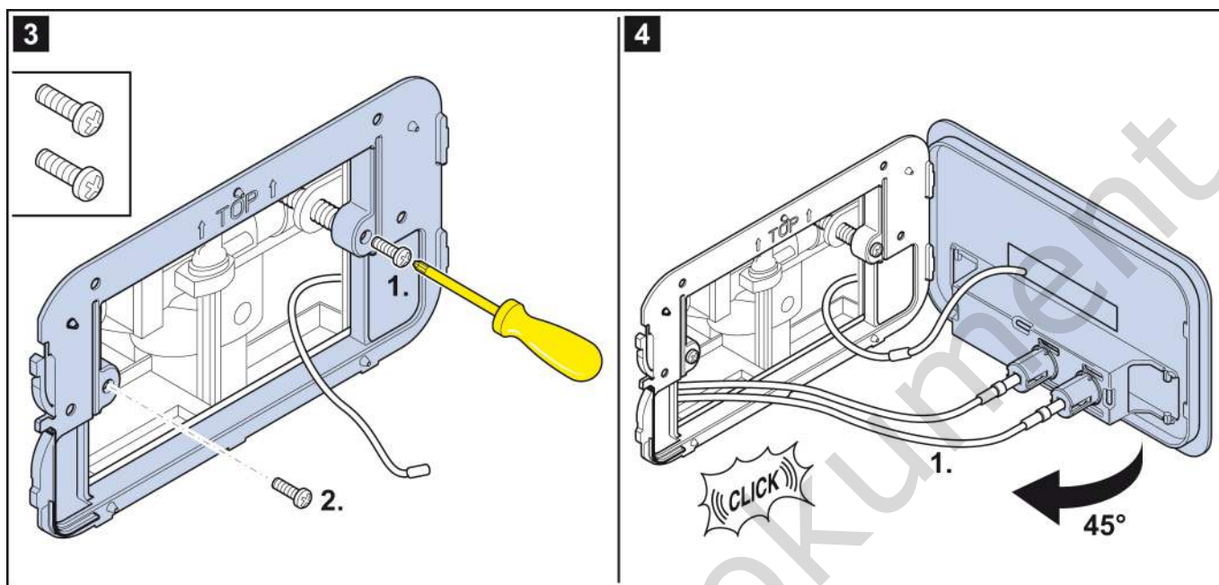
3. Install push plate, see Illustration 5.
