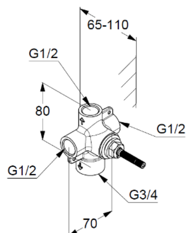
Dimensional drawing
