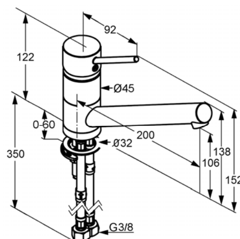
Dimensional drawing
