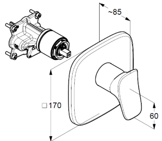
Dimensional drawing
