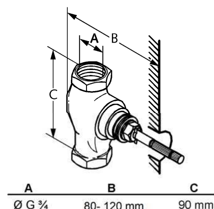
Dimensional drawing
