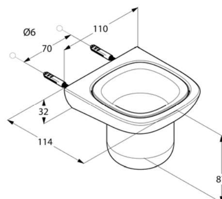
Dimensional drawing
