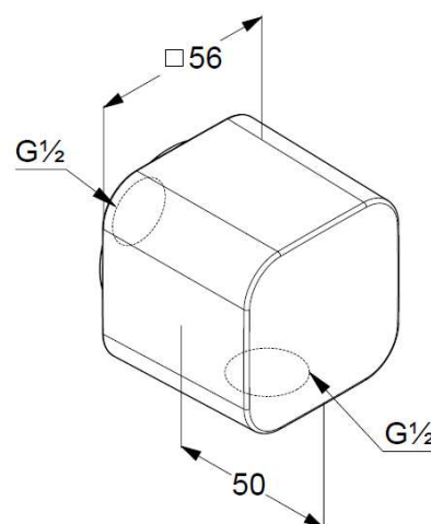
Dimensional drawing
