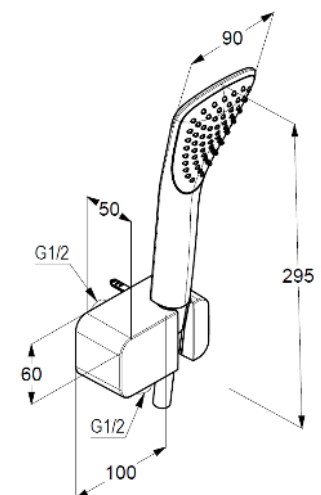
Dimensional drawing
