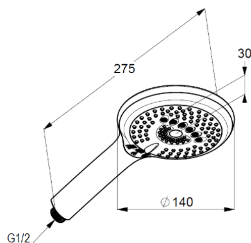
Dimensional drawing
