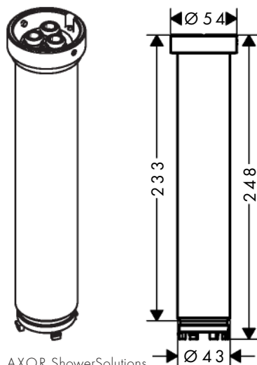
AXOR ShowerSolutions 35288XXX
