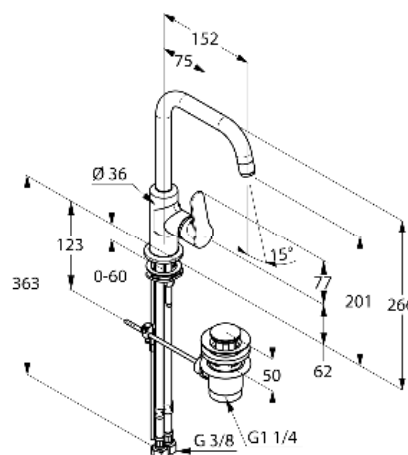
Dimensional drawing
