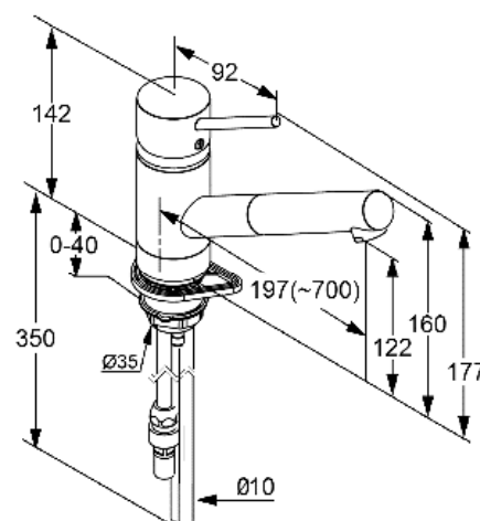
Dimensional drawing
