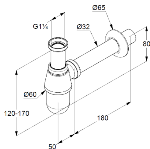
Dimensional drawing
