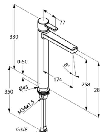
Dimensional drawing
