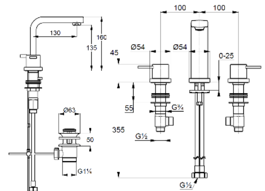
Dimensional drawing
