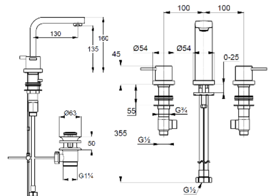
Dimensional drawing
