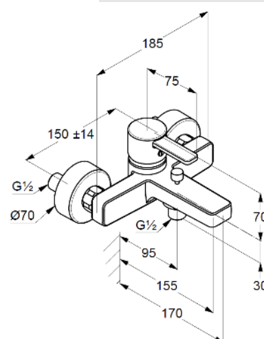
Dimensional drawing
