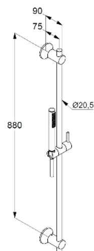
Dimensional drawing
