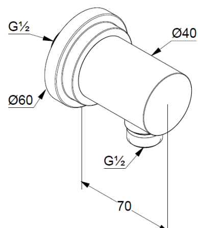
Dimensional drawing
