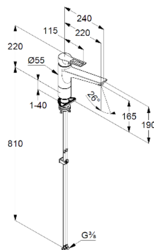
Dimensional drawing
