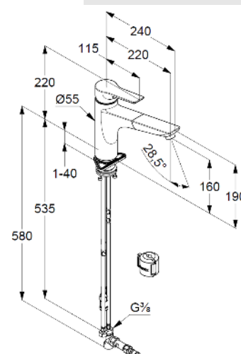
Dimensional drawing
