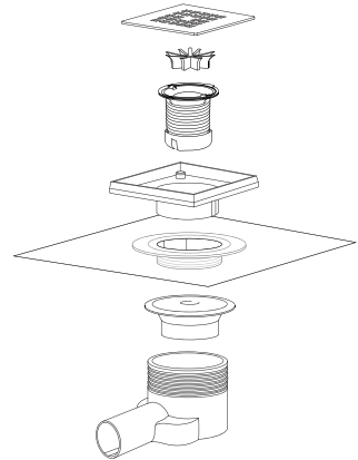
Raindrain Point 56246800 / 56248800
