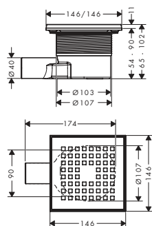
Raindrain Point 56248800
