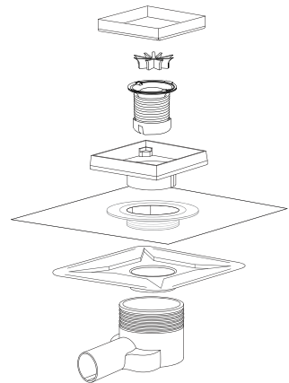
Raindrain Point 56247800 / 56247670 / 56249800 / 56249670
