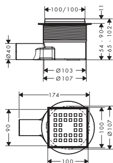
Raindrain Point 56246800
