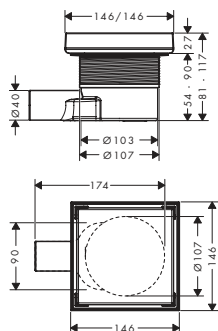
Raindrain Point 56249800 / 56249670
