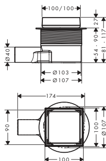
Raindrain Point 56247800 / 56247670
