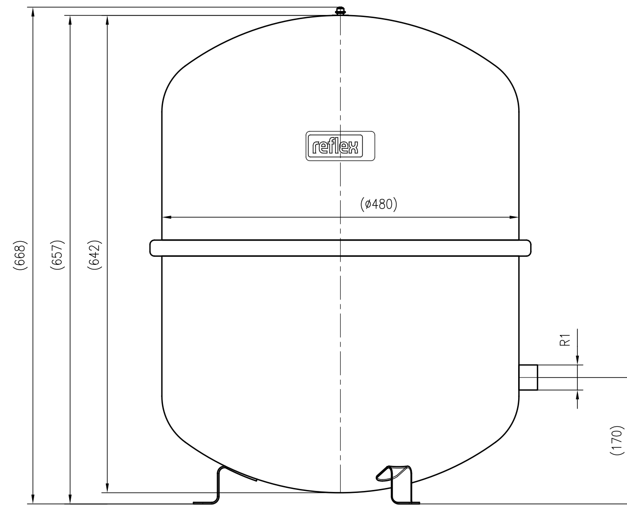
Front view
