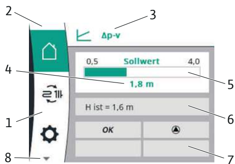
Fig. 7: Homescreen
