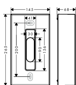
AXOR Universal Circular 42873XX0
