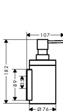
AXOR Universal Circular 42810XX0
