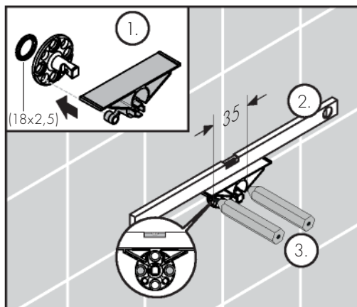
AXOR Universal Circular 42822XX0
