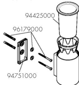
AXOR Universal Circular 42804XX0
