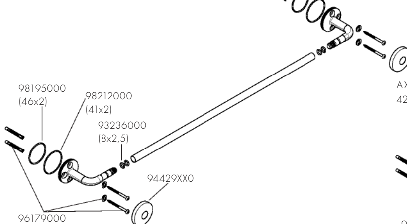
AXOR Universal Circular 42860XX0/42880XX0
