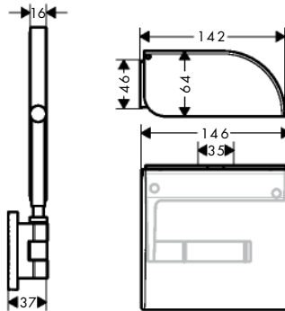
AXOR Universal Circular 42858XX0
