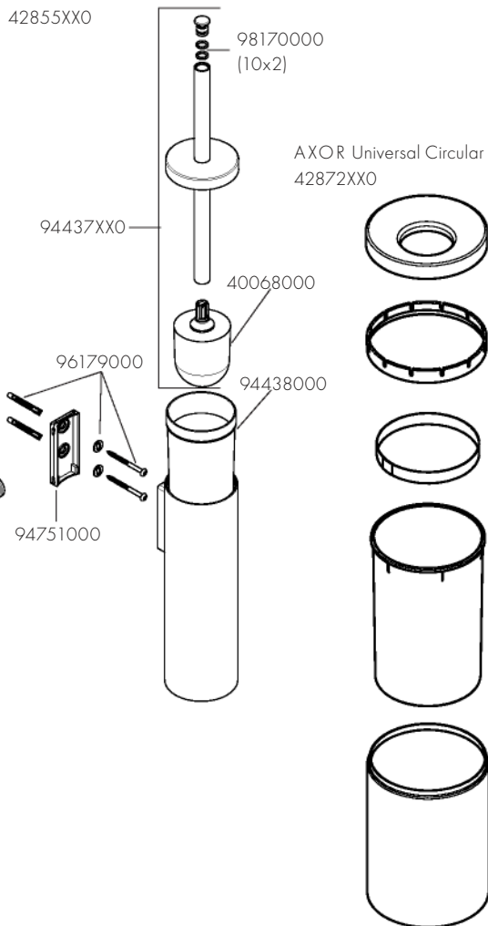
AXOR Universal Circular 42855XX0
