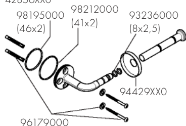
AXOR Universal Circular 42856XX0
