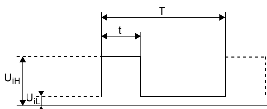
Abb. 49 PBM-Signal
