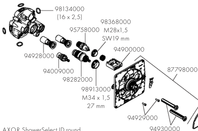
AXOR ShowerSelect ID round 36756XX0
