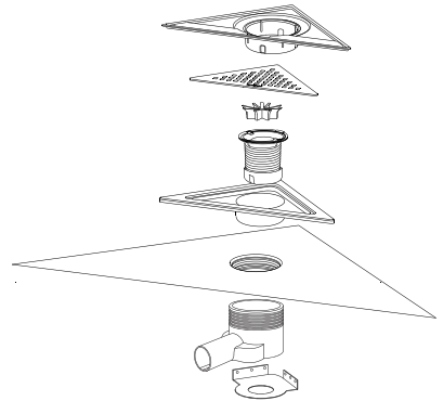
Raindrain Corner 56252800
