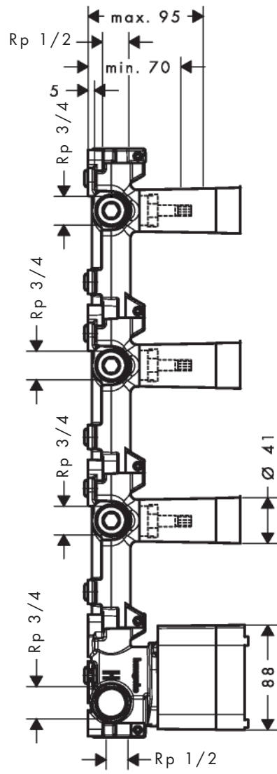
AXOR One 48720180
